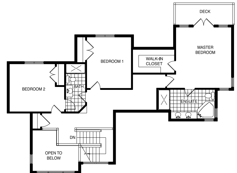
UPPER: 1,220 SQ. FT.
